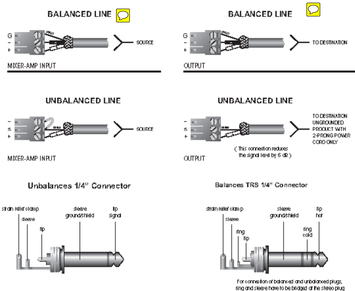
[ Figure 2.1 Input wire and connectors ]
