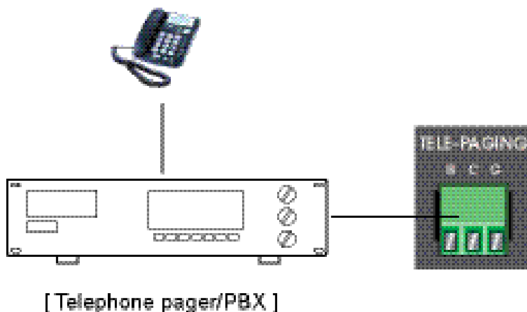
[ Figure 3.1 Telephone paging connection ]
